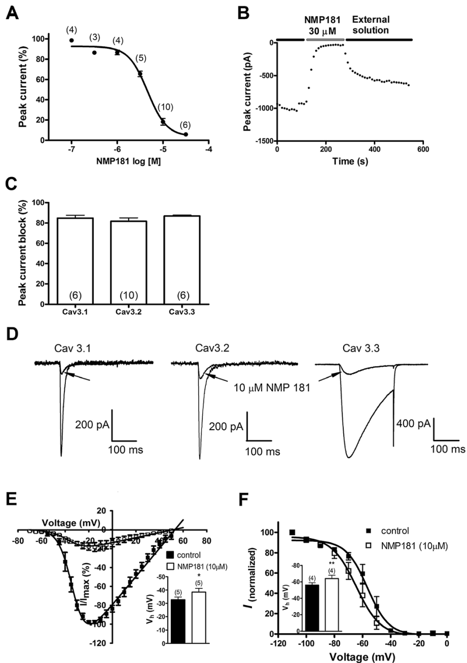
Figure 2 Pharmacological and biophysical properties of NMP-181 block of T-type calcium channels. (A) concentration dependence of NMP-181 inhibition of the Ca_v3.2 peak current amplitude. The data were fitted with a Hill equation. The half-maximal inhibitory concentration ( IC_{50} ) from the fit was 4.6 \mu M and the Hill coefficient was 2.1. Numbers in parentheses reflect numbers of experiments for each concentration point. (B) representative time course of the development of and recovery from NMP-181 ( 30 \mu M ) inhibition. (C), NMP-181 ( 10 \mu M ) did not show selectivity on Ca_v3 channels, as illustrated in the histogram and (D) representative traces from NMP-181 inhibition on Ca_v3.1 , 3.2 and 3.3 currents. Statistical significance was determined by one-way ANOVA followed by a Dunnett's test, when the data were compared to those from Ca_v3.2 group. (E) normalized current-voltage relations of Ca_v3.2 current before and after application of 10 \mu M NMP-181. The half-activation potentials were -32.7 \pm 2.0 mV and -38.4 \pm 2.8 mV before and after application of NMP-181, respectively (inset, P < 0.05 , paired t test). (F) steady-state inactivation curve obtained from Ca_v3.2 channels before and after application of 10 \mu M NMP-181. The half-inactivation potentials were -56.0 \pm 2.8 mV and -64.1 \pm 4.0 mV before and after the treatment with NMP-181, respectively (inset, P < 0.01 , paired t test).
